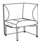
SA810 rak koppling (25) H 850 SH 450 B 665 D 665
