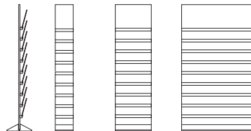
FREB2599 FREB5099 FREB10099 FRET2599* FRET5099** FRET10099*** *incl. 3 magnets **incl. 4 magnets ***incl. 6 magnets
