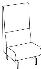
SA510 1-sits 700 H 1405/1435 SH 440/470 B 700 D 700
