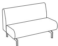
SA410 2-sits, bengavel x 2 H 800/830 SH 440/470 B 1200 D 700
