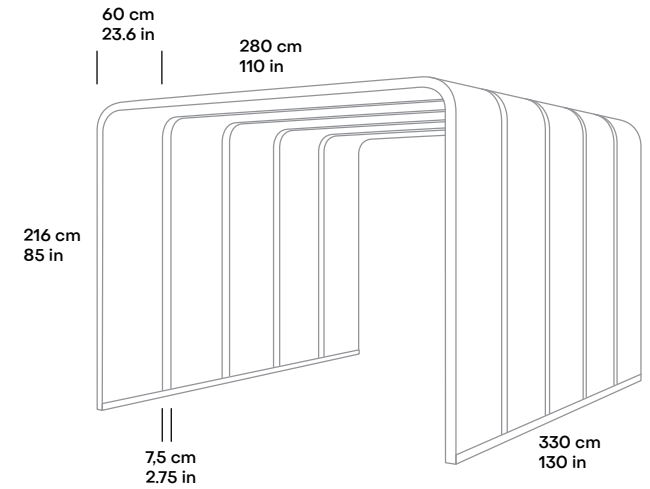
Silen Bridges Portal with 5 arches (W2800)
