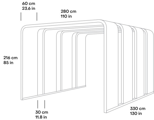
Silen Bridges Portal with 4 arches (W2800)
