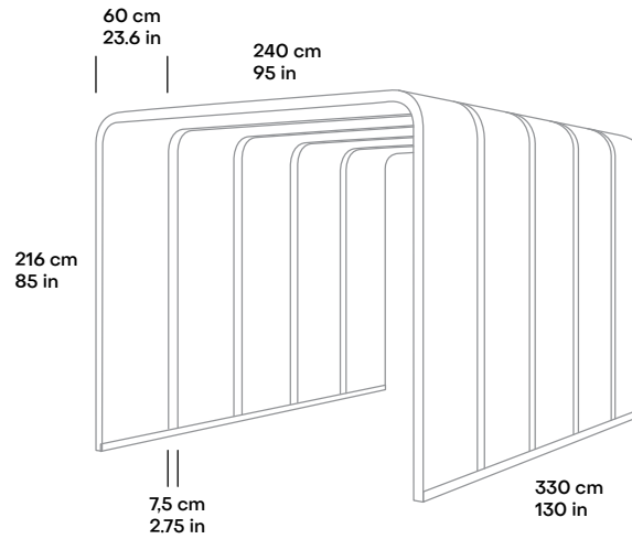
Silen Bridges Portal with 5 arches (W2400)
